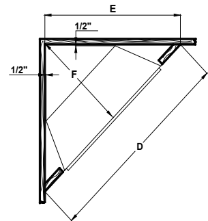
CORNER VIEW
